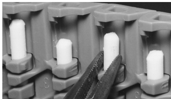
Figure 147: Grip rod
