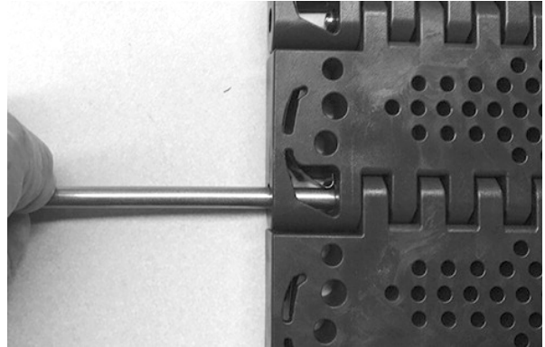
Figure 109: Push rod from belt
