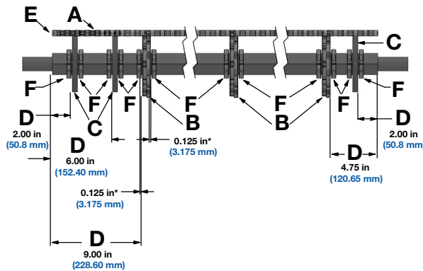
Figure 320: S2600-1.0 > = 26 in (660.4 mm)
