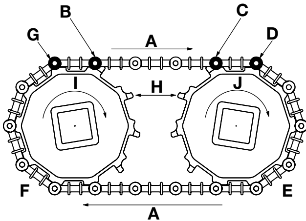
Figure 35: Reverse every other sprocket
