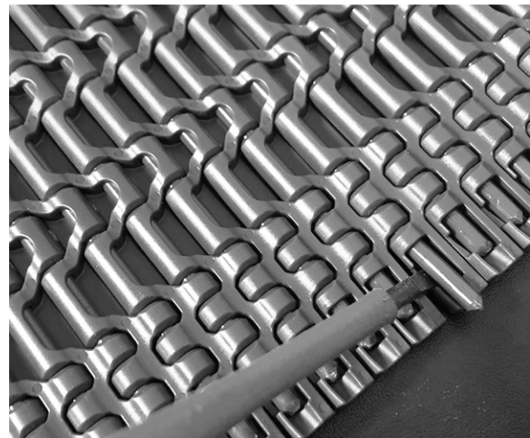
Figure 61: Lift rod over retention feature
