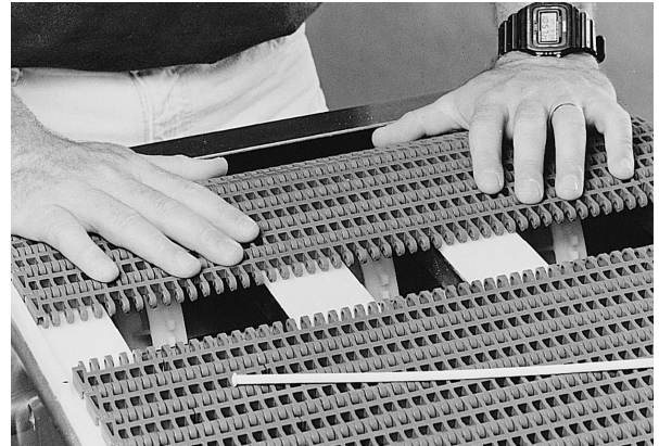
Figure 13: Push belt ends together
