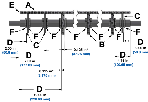
Figure 319: S2600-1.6, 2.2, 2.5, 3.2
