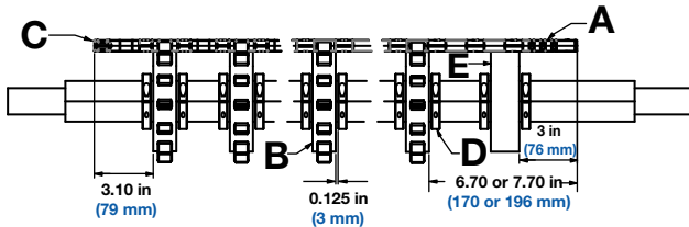
Figure 341: Belt width of 24 in (610 mm) and less
