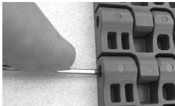
Figure 130: Push rod past belt edge
