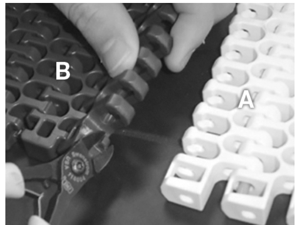
Figure 294: Trim rod guides from old design module (B)
