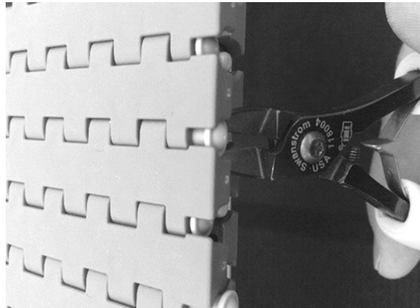
Figure 134: Cut rod head
