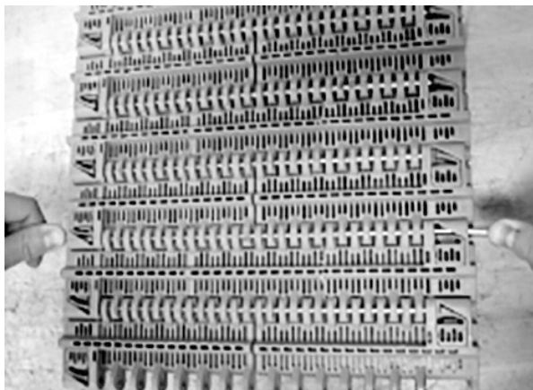
Figure 106: Pull rod from belt
