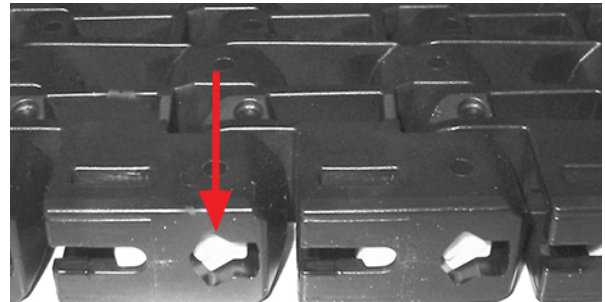
Figure 187: Open Slidelox
