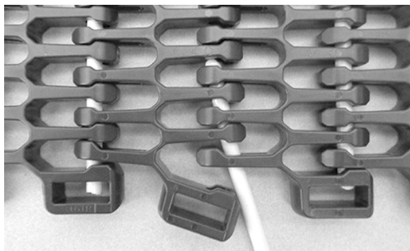
Figure 323: Insert rod through hinges
