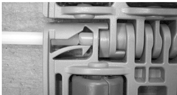
Figure 222: Push rod past retention feature
