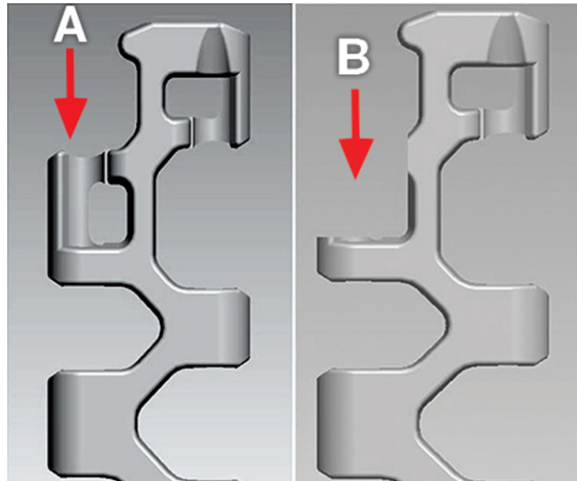
Figure 172: Cut retention feature
