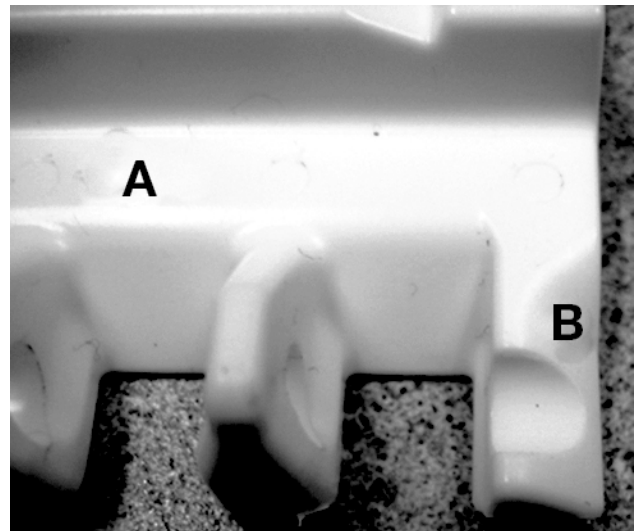
Figure 73: Original Flush Edge hinges
