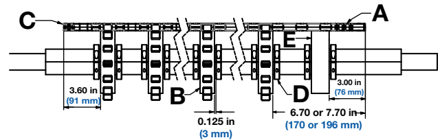
Figure 344: Belt width of 16 in (407 mm) and less
