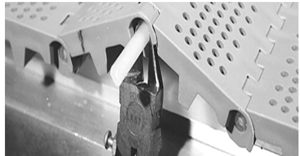
Figure 65: Cut rod flush with belt edge
