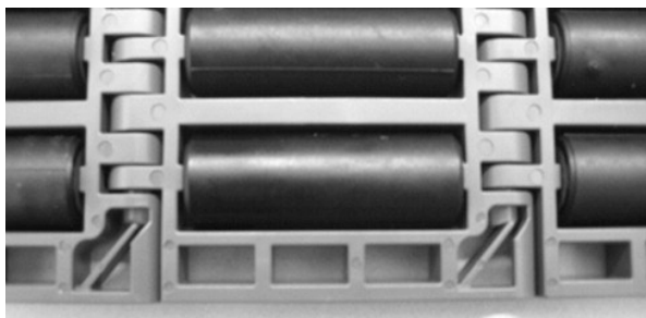
Figure 238: Ensure rod is past retention feature
