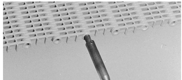
Figure 30: Close rod hole
