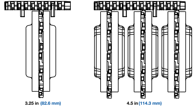
Figure 115: Sprocket tracking tabs
