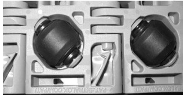
Figure 232: Ensure rod is past retention feature
