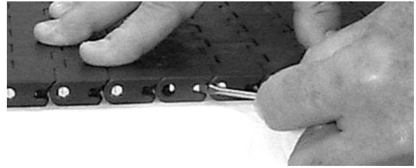
Figure 165: Close Slidelox
