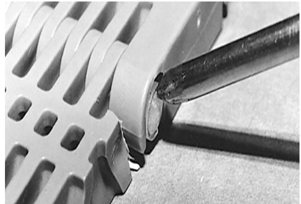
Figure 48: Push rod head past retention feature
