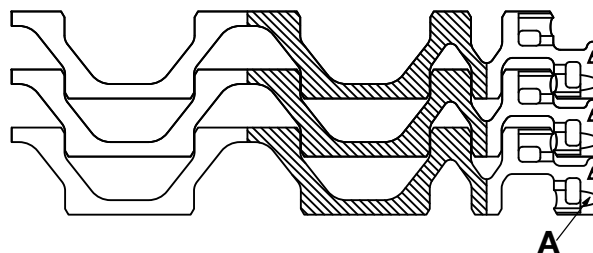
A Insertion guide notch Figure 168: Use insertion guide notch as guide
