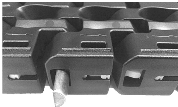
Figure 199: Insert rod
