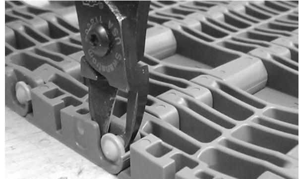
Figure 268: Cut rodlet
