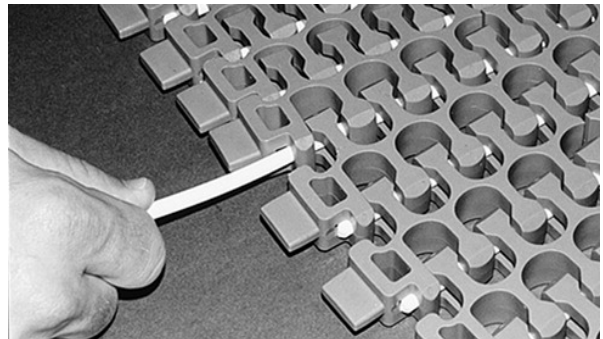
Figure 270: Insert rod
