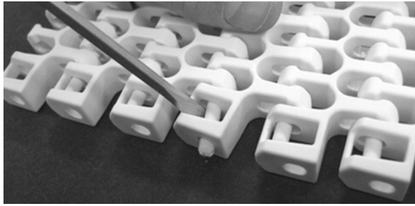
Figure 290: Push rod through retention feature
