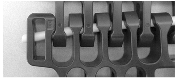
Figure 314: Push rod past retention feature
