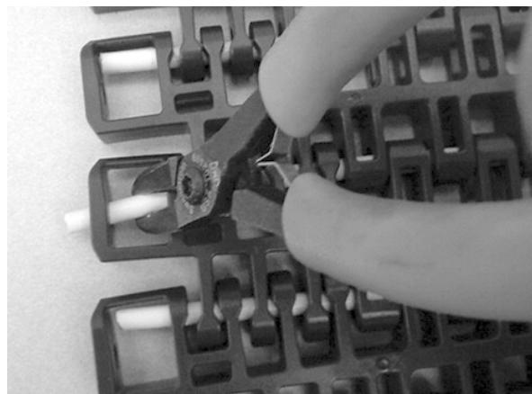
Figure 357: Push rod past retention feature
