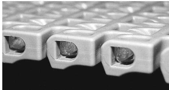
Figure 146: Ensure rod is past retention feature
