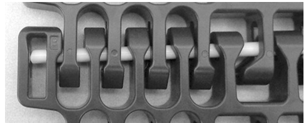
Figure 315: Ensure rod is past retention feature
