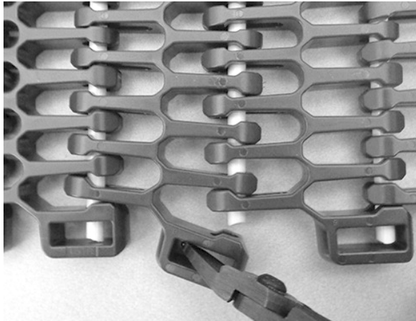
Figure 327: Flex flush edge of module
