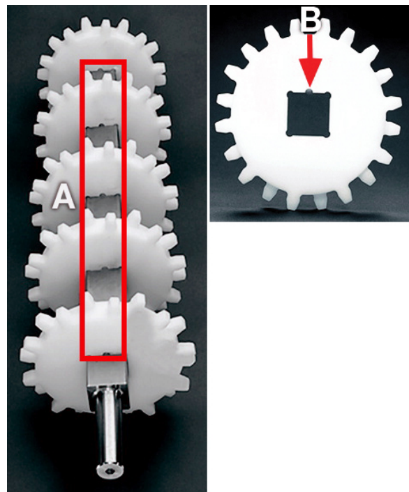
A Notches aligned B Sprocket alignment notches
