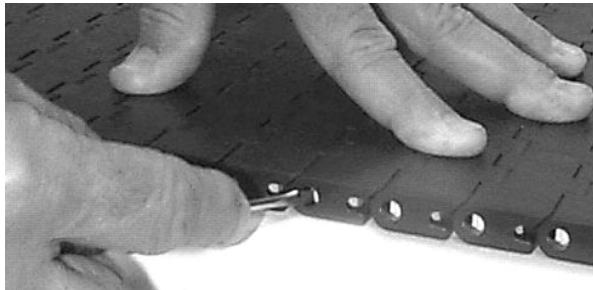
Figure 163: Open Slidelox
