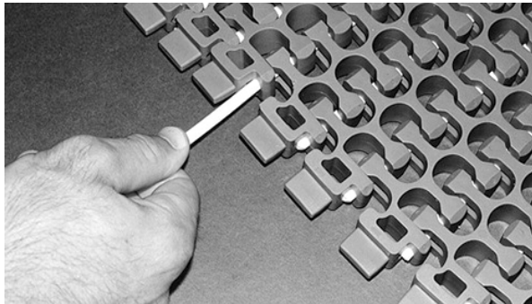
Figure 275: Pull out rod
