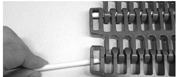
Figure 330: Insert rod
