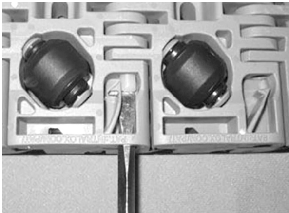
Figure 231: Push rod past retention feature
