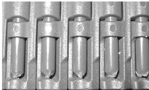
Figure 55: Ensure rod is past retention feature
