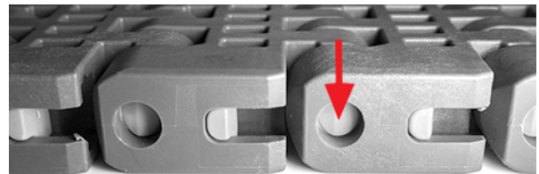
Figure 155: Ensure Slidelox is open
