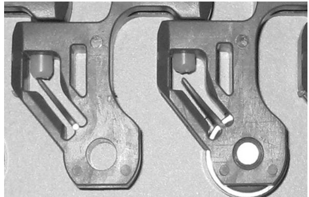
Figure 301: Ensure rod is past retention feature
