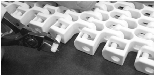
Figure 291: Pull rod from belt
