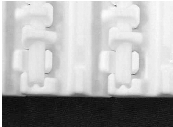
Figure 175: Ensure rod is past retention feature
