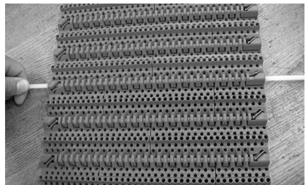
Figure 87: Pull rod from belt
