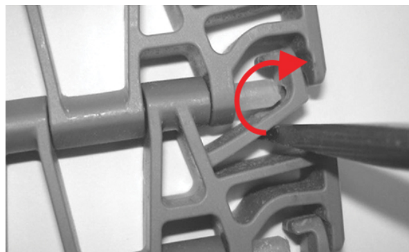
Figure 249: Rotate screwdriver to hold retention feature open
