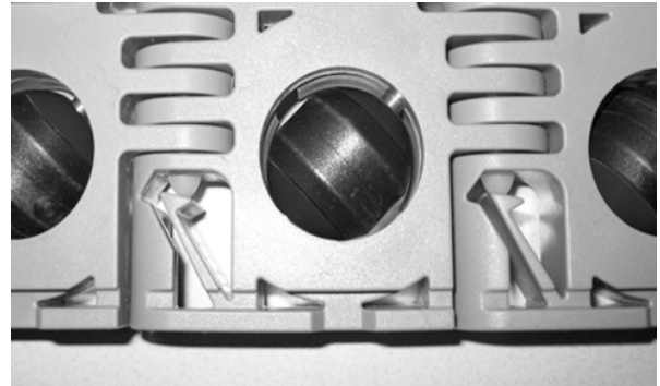
Figure 51: Ensure retention feature
