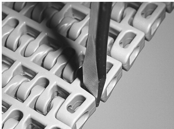
Figure 138: Push rod past retention feature
