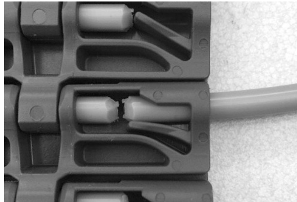
Figure 129: Push retention feature open
