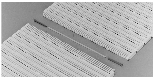
Figure 21: Abrasion resistant rod and rodlets
