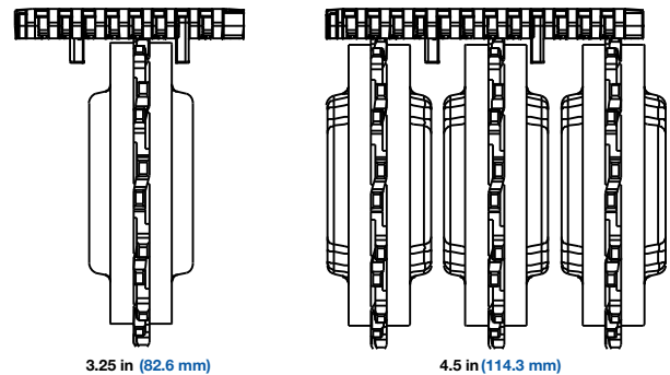
Figure 166: Sprocket tracking tabs
