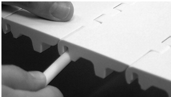
Figure 203: Insert rod through hinges
