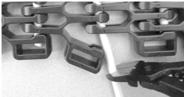
Figure 329: Pull rod from belt
