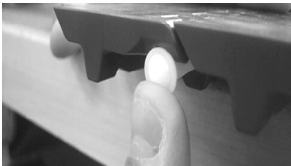
Figure 97: Use thumb to push rod
