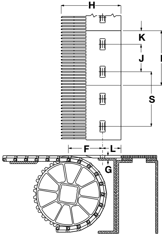
Figure 19: Finger transfer plates location
