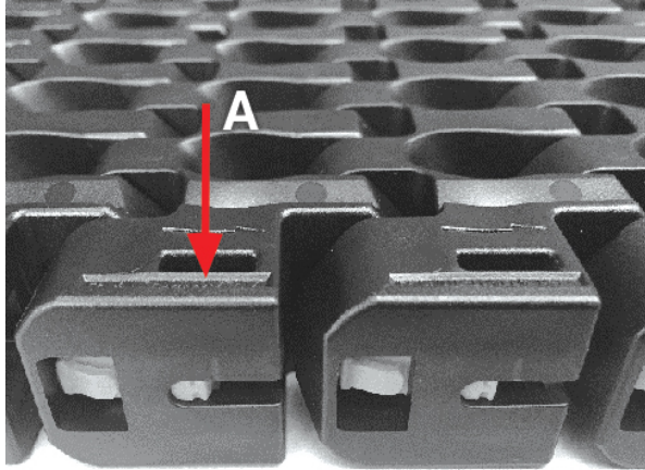
Figure 201: Open Slidelox
