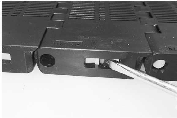
Figure 212: Open Slidelox
