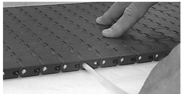
Figure 161: Insert rod
