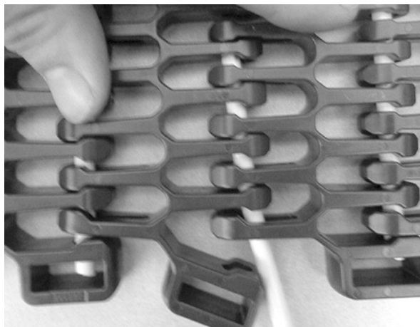
Figure 324: Align hinges
