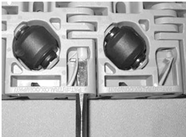
Figure 225: Push rod past retention feature
