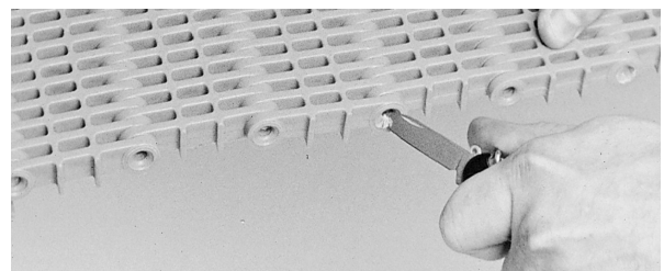
Figure 31: Open rod hole
