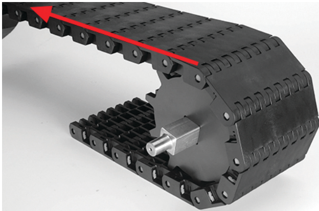
Figure 264: Slidex on left
