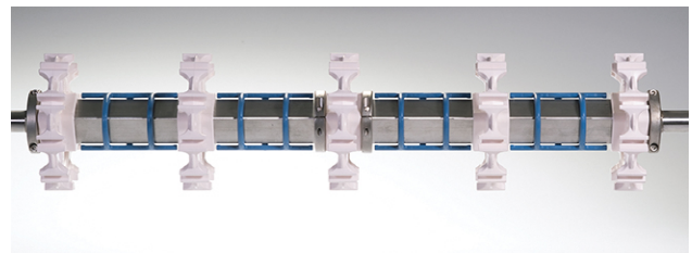
Figure 91: Sprocket spacer on shaft
