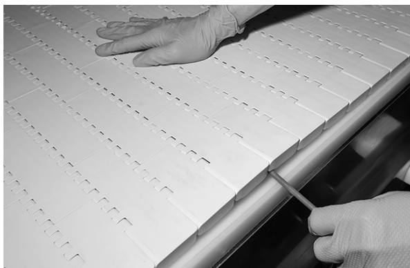
Figure 89: Push rod through the hinges until fully seated
