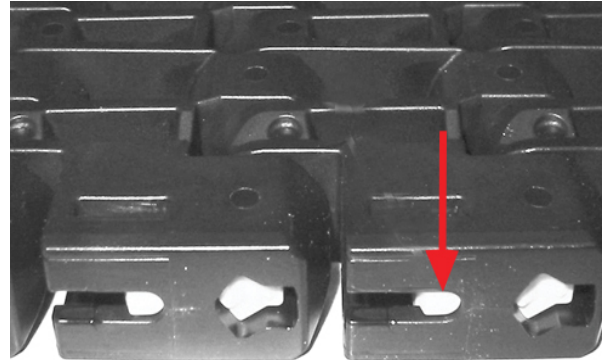
Figure 186: Close Slidelox
