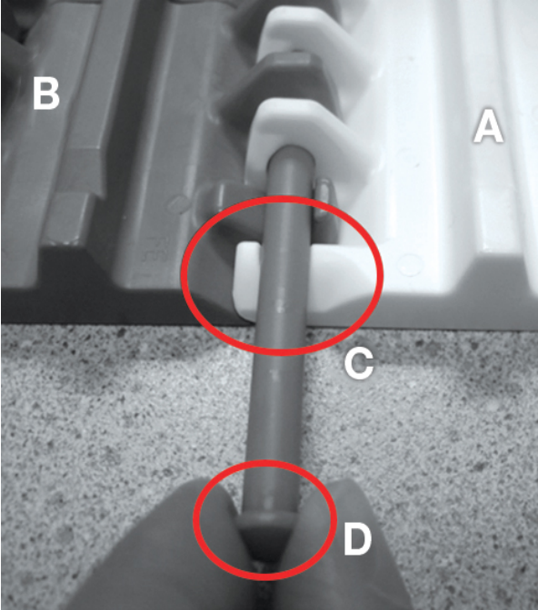
A Updated design B Original design C New rod retention geometry D Rod head
