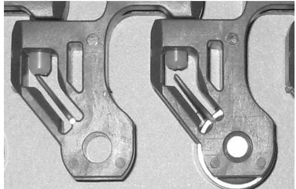
Figure 279: Ensure rod is past retention feature
