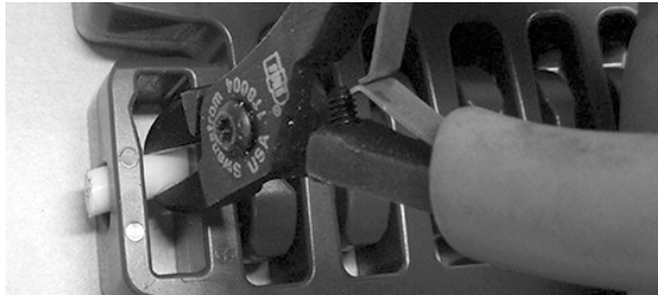
Figure 333: Push rod to side and past occluded hole
