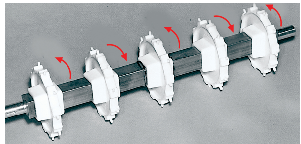
Figure 35: Reverse every other sprocket
