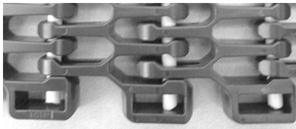
Figure 326: Ensure rod is fully inserted
