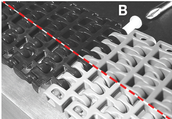
Figure 141: Push rod past older module edge
