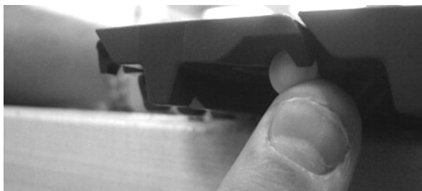
Figure 98: Push rod past retention feature
