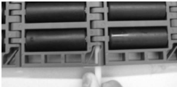
Figure 236: Insert rod through hinges
