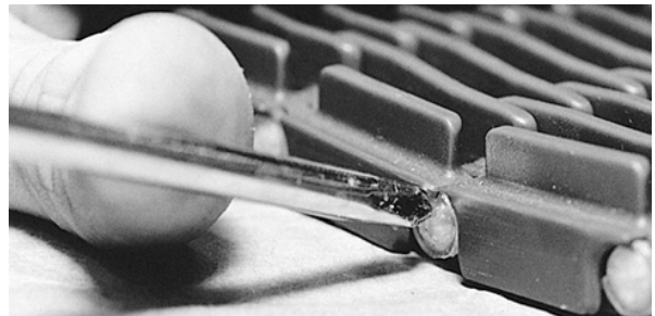
Figure 112: Ensure rod is past snap-lock
