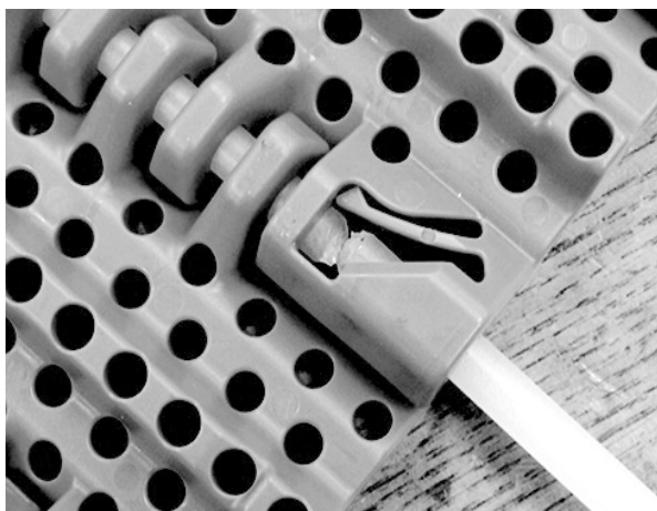
Figure 85: Push rod past retention feature
