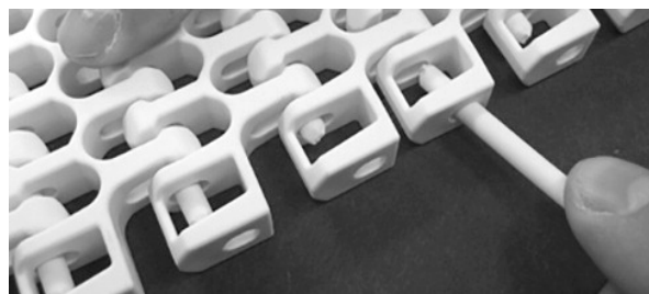
Figure 287: Insert rod through hinges
