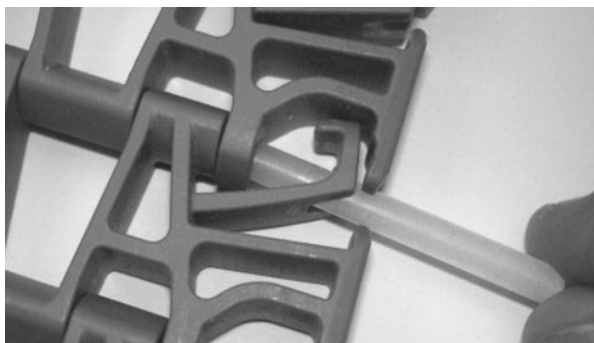
Figure 246: Insert rod through hinges
