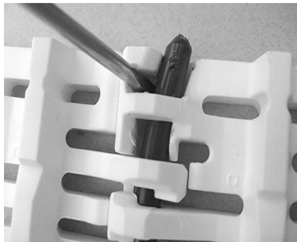
Figure 82: Lift rod past retention feature
