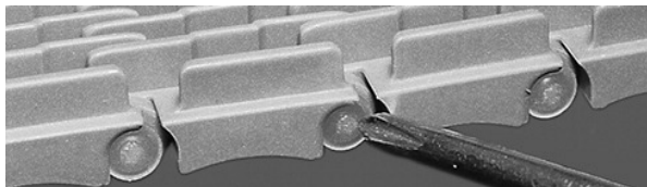
Figure 23: Ensure rod head is past snap-lock
