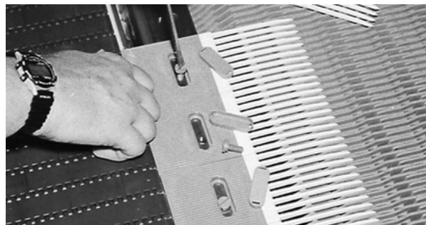
Figure 18: Install finger transfer plates using Intralox plastic bolts
