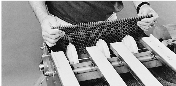
Figure 11: Feed belt down returnway
