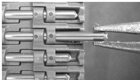
Figure 57: Pull rod from belt
