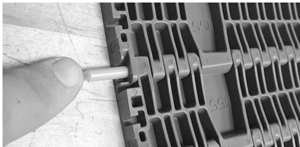
Figure 266: Insert rod
