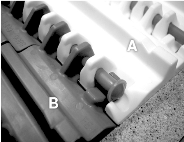
A Updated design B Original design
