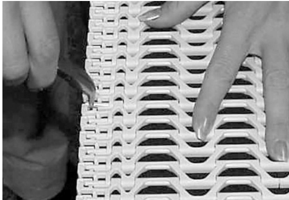
Figure 171: Pull rod from belt
