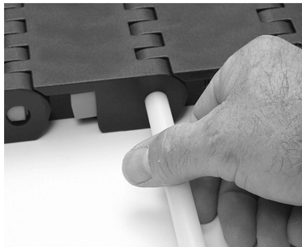
Figure 258: Insert rod
