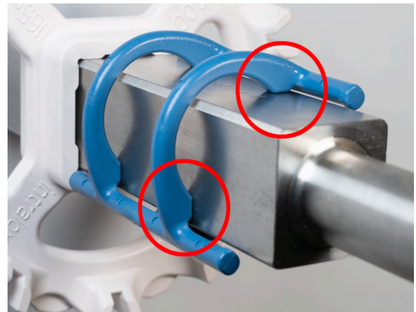
Figure 93: Ensure spacer is flat against shaft
