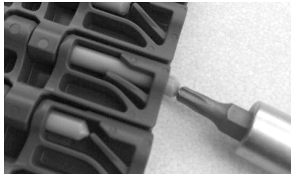
Figure 128: Push rod past retention feature
