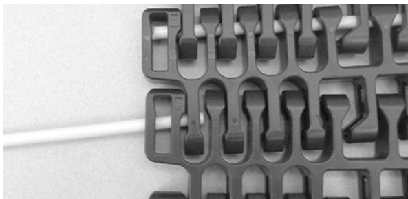
Figure 313: Insert rod
