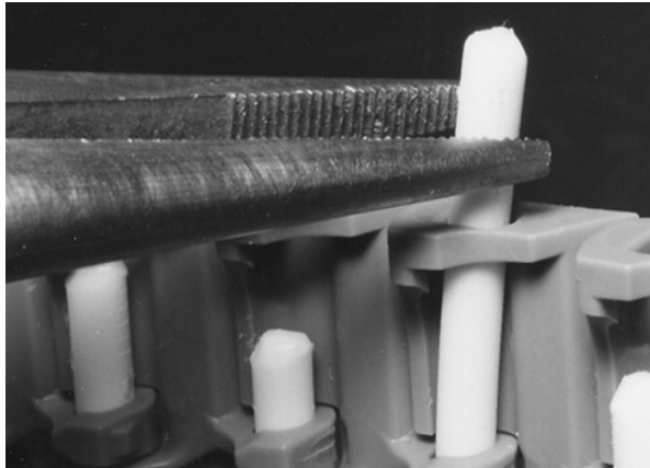
Figure 149: Pull rod from belt
