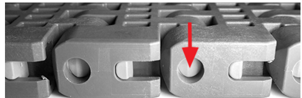
Figure 157: Open Slidelox
