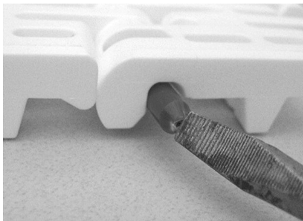
Figure 80: Push rod past retention feature
