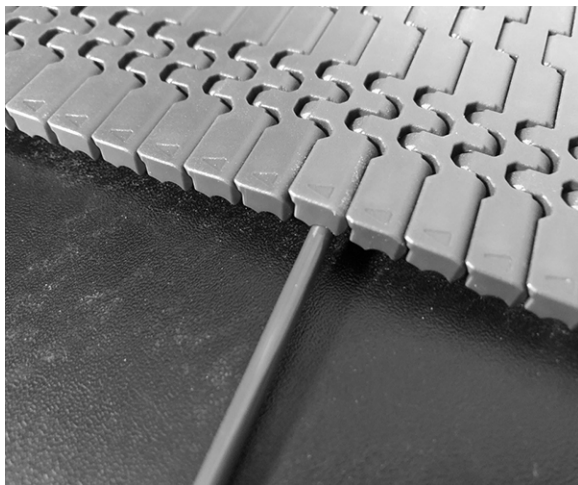
Figure 58: Insert rod
