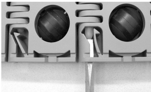
Figure 50: Push rod past retention feature
