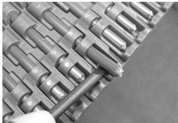
Figure 56: Lift rod over retention feature
