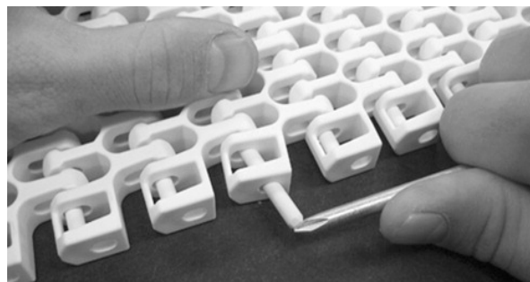
Figure 288: Push rod past retention feature
