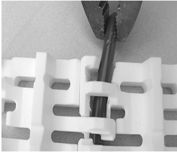
Figure 83: Pull rod from belt
