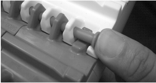
Figure 77: Push rod past retention feature
