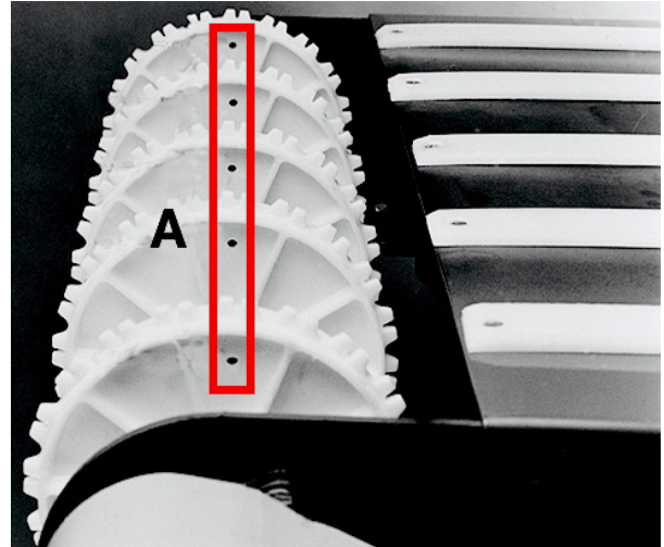
A Ensure pilot holes are aligned Figure 2: Shaft with aligned sprockets
