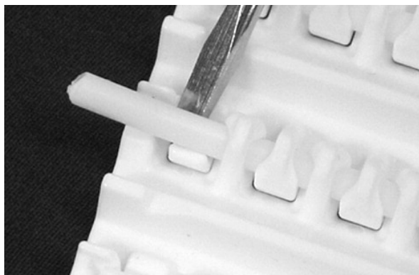
Figure 176: Lift rod over retention feature
