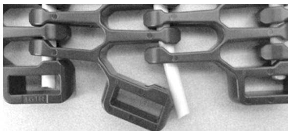
Figure 325: Push rod past belt edge
