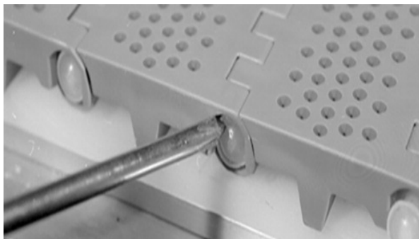
Figure 64: Ensure rod head is past snap-lock
