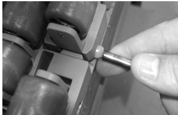
Figure 190: Push rod past retention feature
