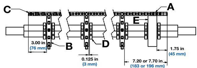
Figure 361: Belt width of 16 in (407 mm) and less
