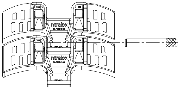
Figure 303: Insert steel pin through hinges
