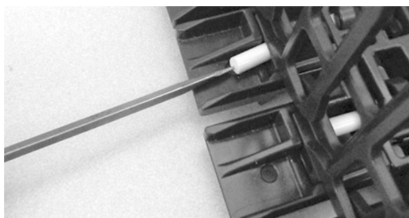
Figure 365: Push rod past retention feature
