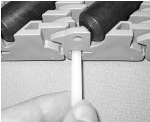
Figure 230: Insert rod through hinges
