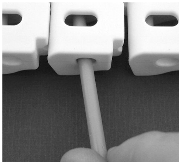
Figure 286: Pull rod from belt
