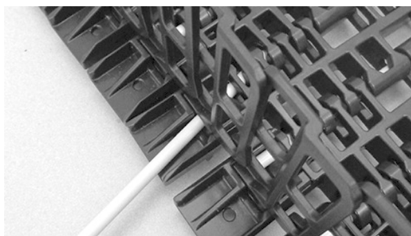
Figure 364: Insert rod through hinges
