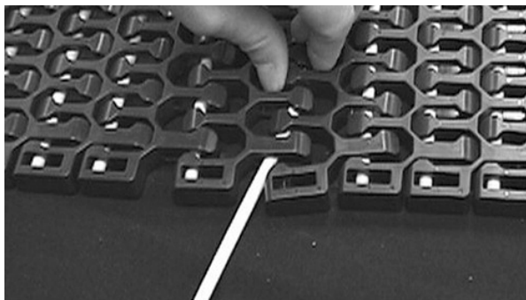
Figure 305: Align hinges
