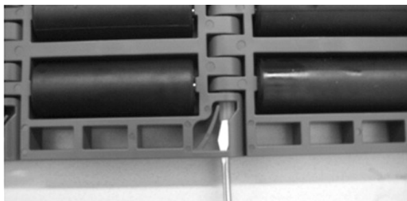
Figure 237: Push rod past retention feature
