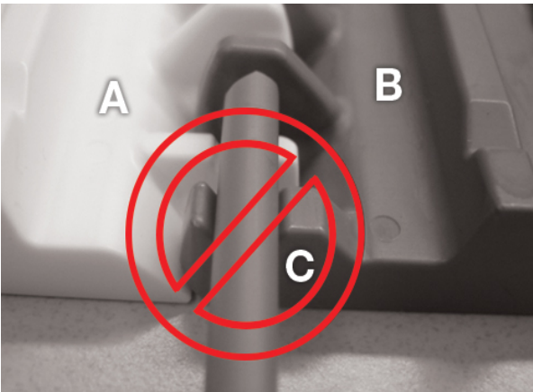
A Updated design B Original design C Old rod retention geometry
