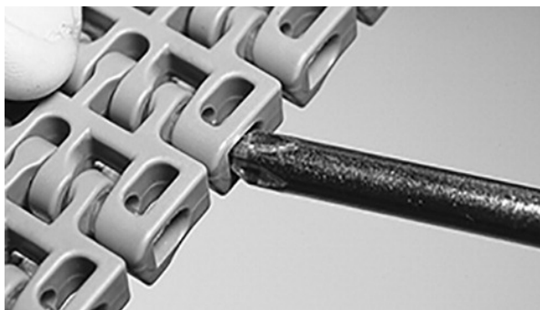
Figure 136: Push rod past retention feature
