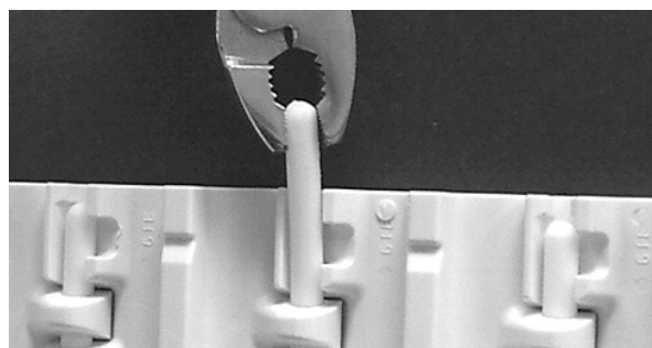
Figure 207: Pull rod from belt
