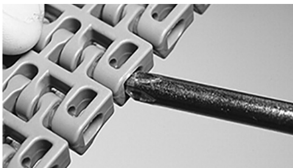
Figure 145: Push rod past retention feature
