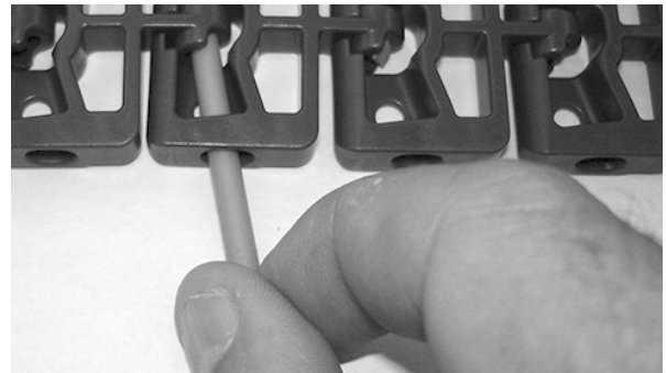
Figure 122: Insert rod through hinges
