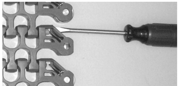
Figure 280: Open retention feature
