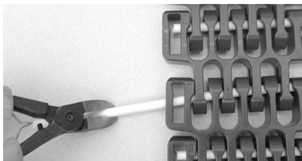
Figure 317: Pull rod from belt
