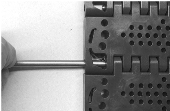
Figure 107: Push rod past retention feature
