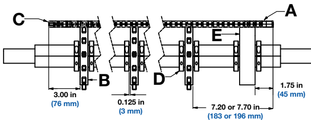
Figure 358: Belt width of 16 in (407 mm) and less
