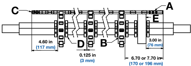
Figure 347: Belt width of 16 in (407 mm) and less
