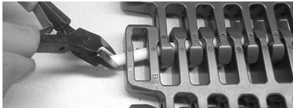
Figure 334: Pull rod from belt
